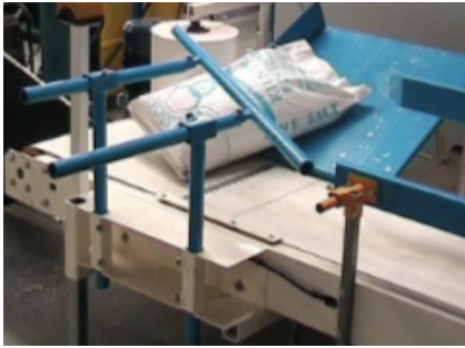
Innotran I Inline turner transferring the bag bottom first.
